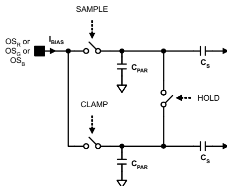
Figure 11. CDS Mode Input Bias Current
