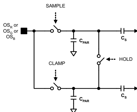
Figure 10. CDS Mode Simplified Input Diagram
