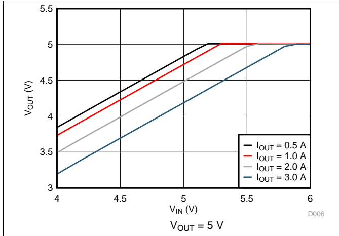
Figure 7. Dropout Curve
