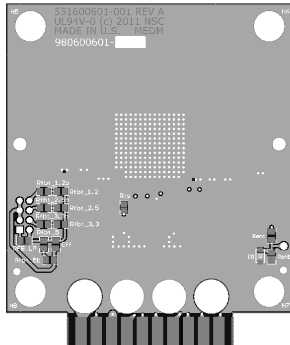
Figure 59. Bottom View of Evaluation PCB
