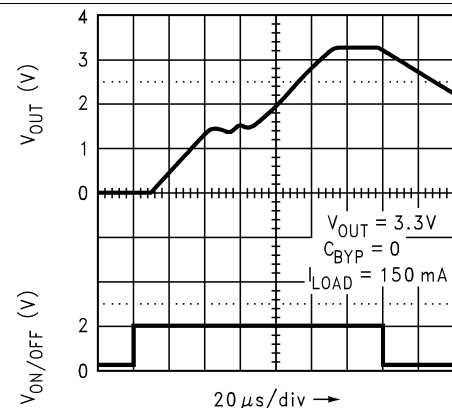
Figure 30. Turnon Time
