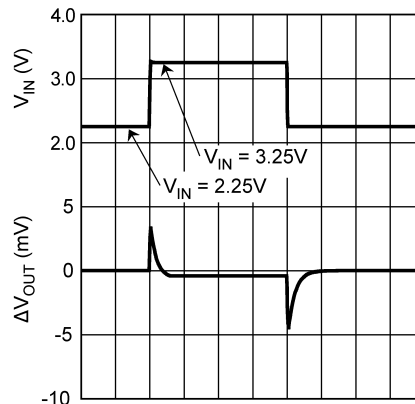
Figure 23. Line Transient
