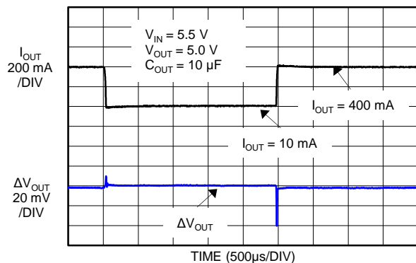
Figure 34. Load Transient
