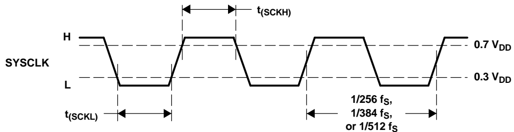
Figure 44. System Clock Timing
