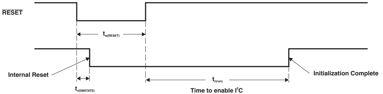
Figure 8-9. Reset Timing
