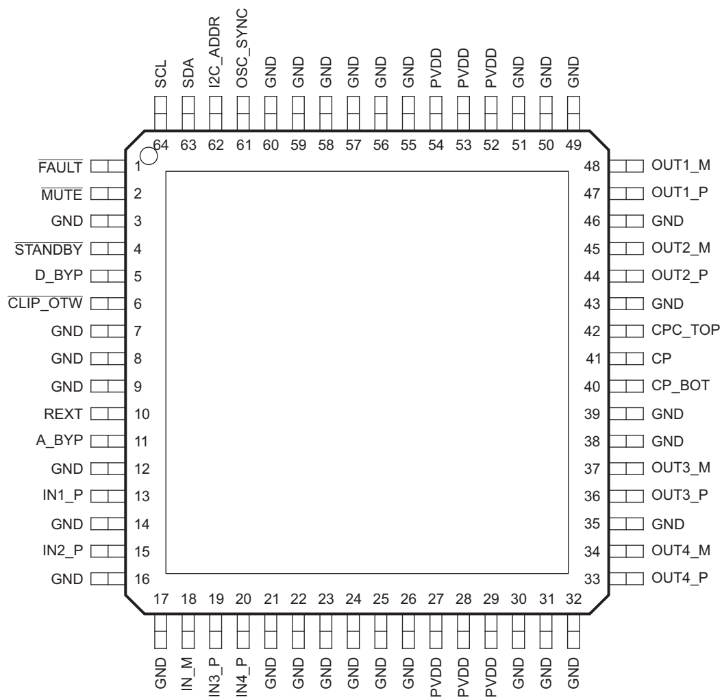
TAS5414B PHD Package (Top View)
