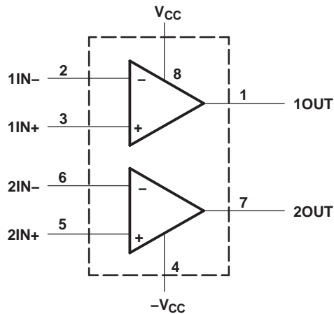
Figure 51. THS4032 – Dual Channel
