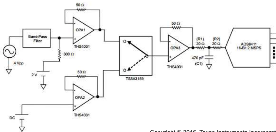
Figure 60. Evaluation Set-Up
