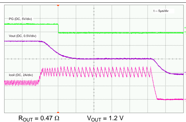
Figure 21. Output Short-Circuit Protection, HICCUP Zoom In
