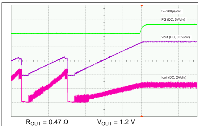
Figure 20. Output Short-Circuit Protection, Recovery
