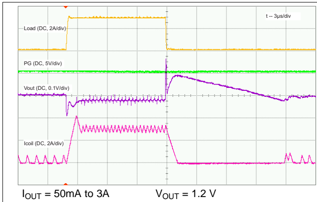
Figure 18. Load Transient
