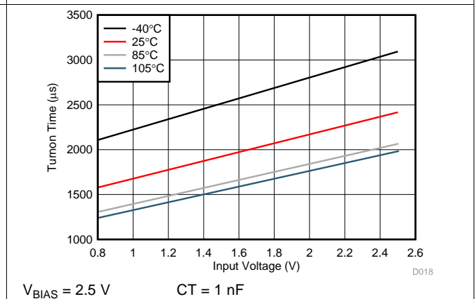
Figure 18. Turnon Time vs Input Voltage
