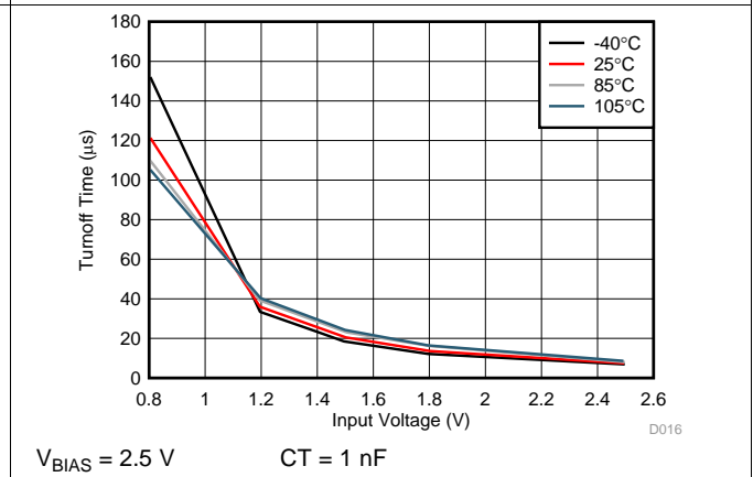
Figure 16. Turnoff Time vs Input Voltage
