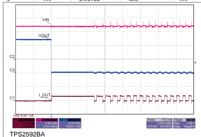
Figure 31. Transient: Thermal Fault Auto-Retry
