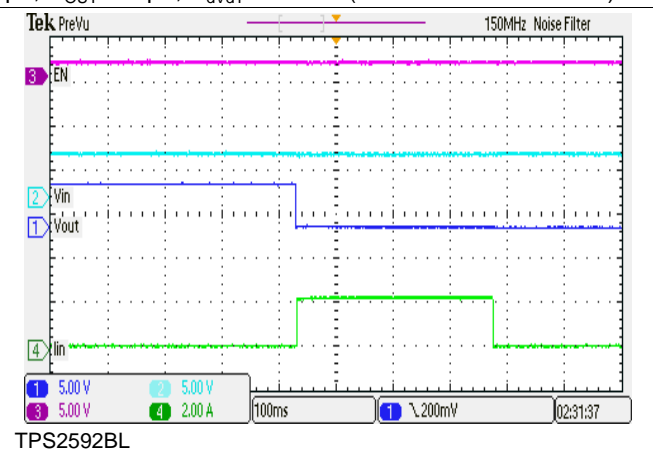
Figure 32. Transient: Thermal Fault Latched
