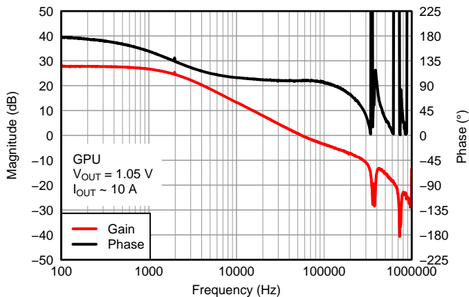
Figure 53. Bode Plot
