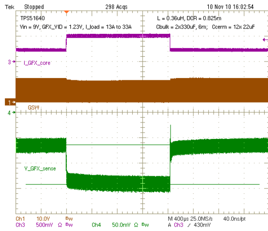
Figure 45. Load Transient, V_{IN} = 9\text{ V} , Load Step = 20 A
