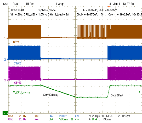
Figure 15. SetVID-Decay/SetVID-Slow
