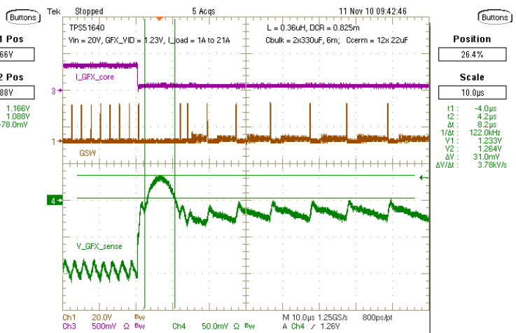
Figure 48. Load Release, V_{IN} = 20\text{ V} , Load Step = 20 A
