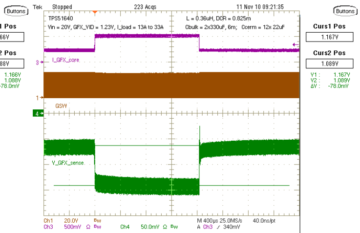
Figure 46. Load Transient, V_{IN} = 20\text{ V} , Load Step = 20 A
