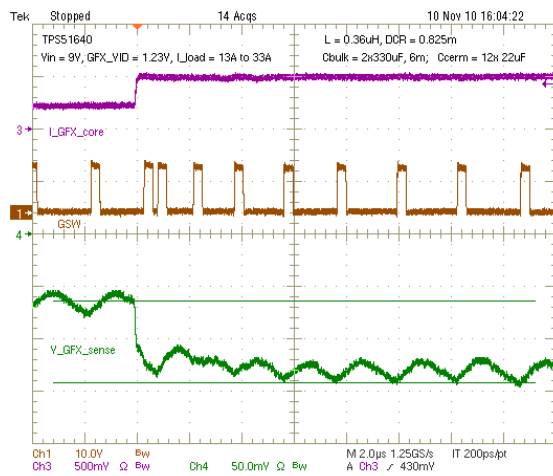
Figure 47. Load Insertion, V_{IN} = 9\text{ V} , Load Step = 20 A
