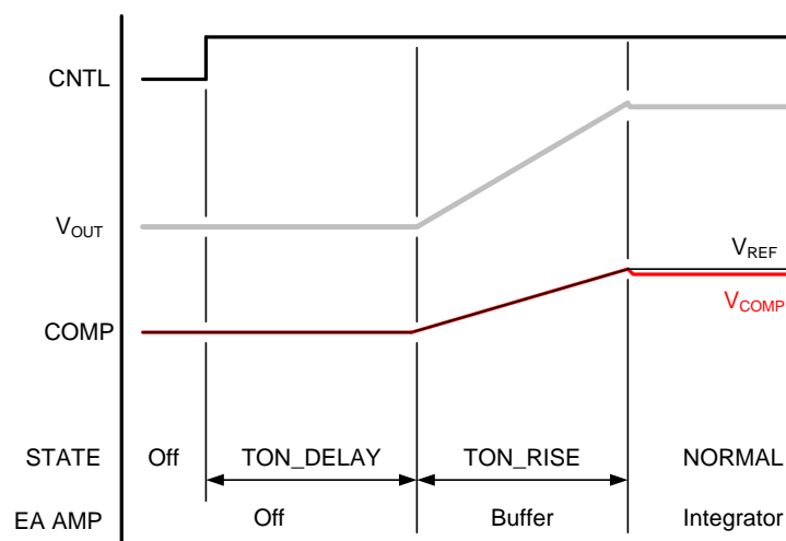
Figure 23. Soft-Start
