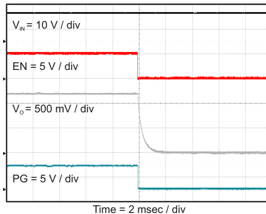
Figure 39. Shut Down Relative to EN Falling
