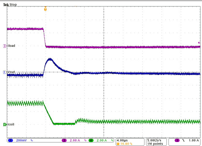
Figure 39. Load Transient Response of Figure 37, Falling Edge
