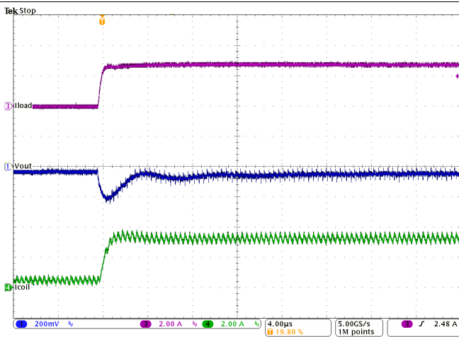
Figure 38. Load Transient Response of Figure 37, Rising Edge
