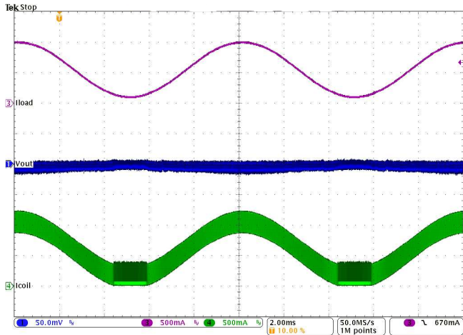
Figure 36. PWM-PSM-Transition
