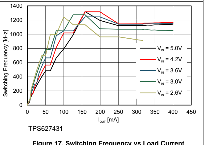
Figure 17. Switching Frequency vs Load Current V_{OUT} = 1.4 V
