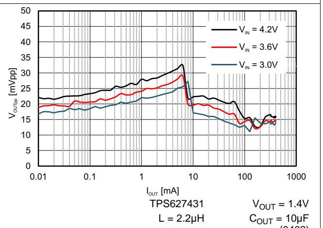
Figure 19. Typical Output Ripple Voltage V_{OUT} = 1.4V
