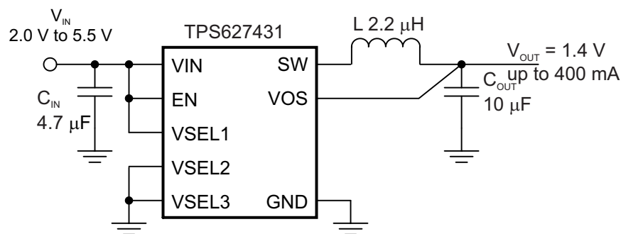
Figure 7. TPS627431 Typical Application Circuit
