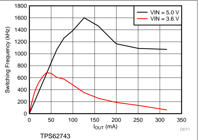
Figure 15. Switching Frequency vs Load Current V_{OUT} = 3.3 V
