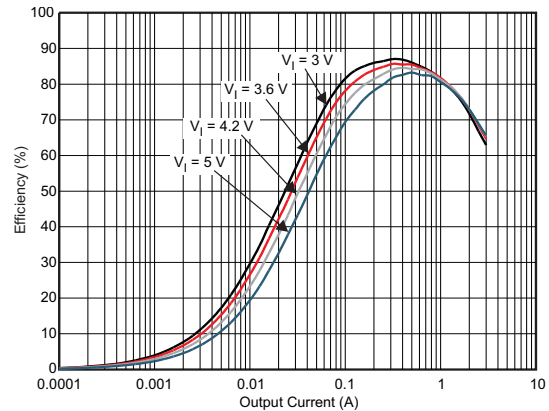
DCDC1 V_O = 0.9\text{ V} PWM Mode DFE252012 25°C
