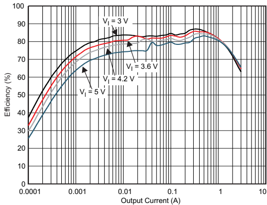
DCDC1 V_O = 0.9\text{ V} PFM Mode DFE252012 25°C
