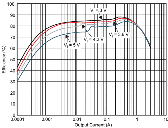
DCDC1 V_O = 1.2\text{ V} PFM Mode LQM2NPN-1 \mu\text{H} 25°C
