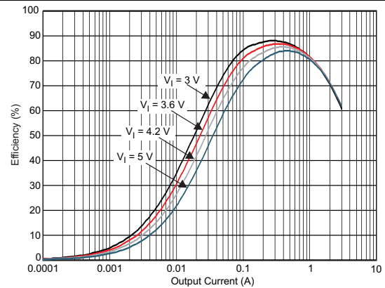
DCDC1 V_O = 1.2\text{ V} PWM Mode LQM2NPN-1 \mu\text{H} 25°C
