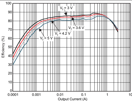
DCDC1 V_O = 1.1375\text{ V} PFM Mode DFE252012 25°C
