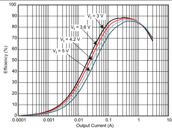
DCDC1 V_O = 1.1375\text{ V} PWM Mode DFE252012 25°C
