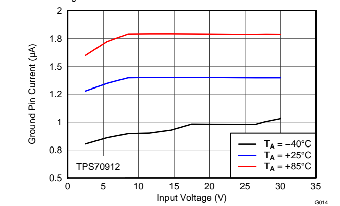
Figure 14. GND Current vs V_{IN} and Temperature
