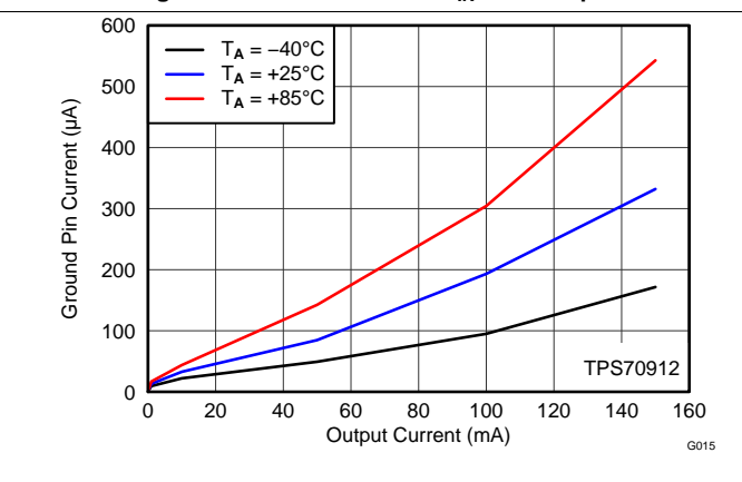
Figure 16. GND Current vs I_{OUT} and Temperature
