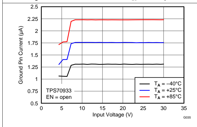
Figure 15. GND Current vs V_{IN} and Temperature
