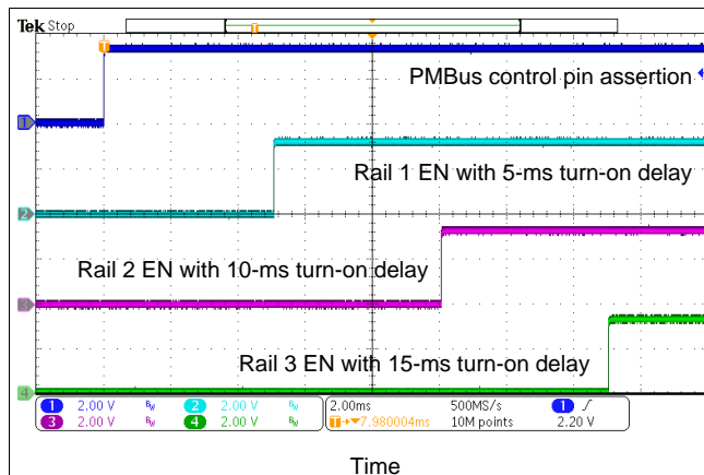
Figure 41. Start-Up Waveforms
