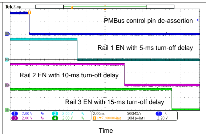
Figure 42. Shut-Down Waveforms
