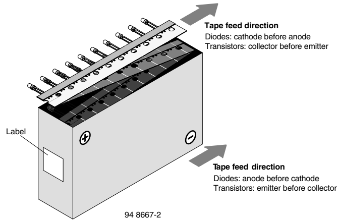
94 8667-2 Fig. 26 - Tape Direction
