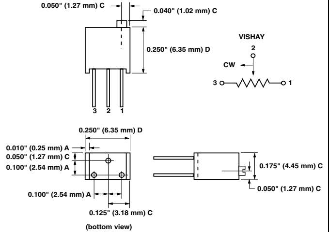
FIGURE 1 - SCHEMATIC AND DIMENSIONS in Inches (Millimeters)
